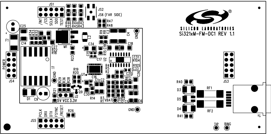
Figure 16. Si321xM-FM-DC1-EVB with Si3201 Primary Assembly
