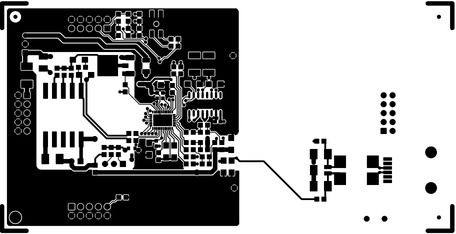
Figure 17. Si321xM-FM-DC1-EVB with Si3201 Primary Side
