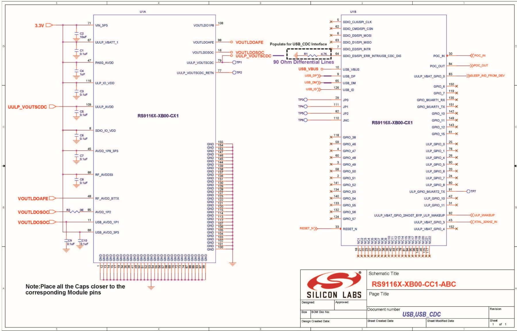
Figure 17. USB Schematics
