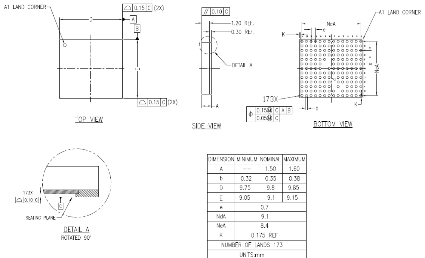
Figure 21. Package Outline
