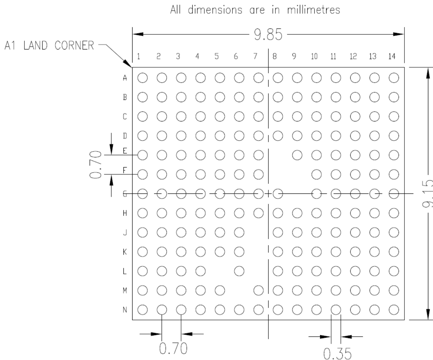
Figure 22. PCB Landing Pattern
