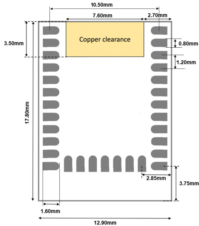
Figure 9.3. Bottom View
