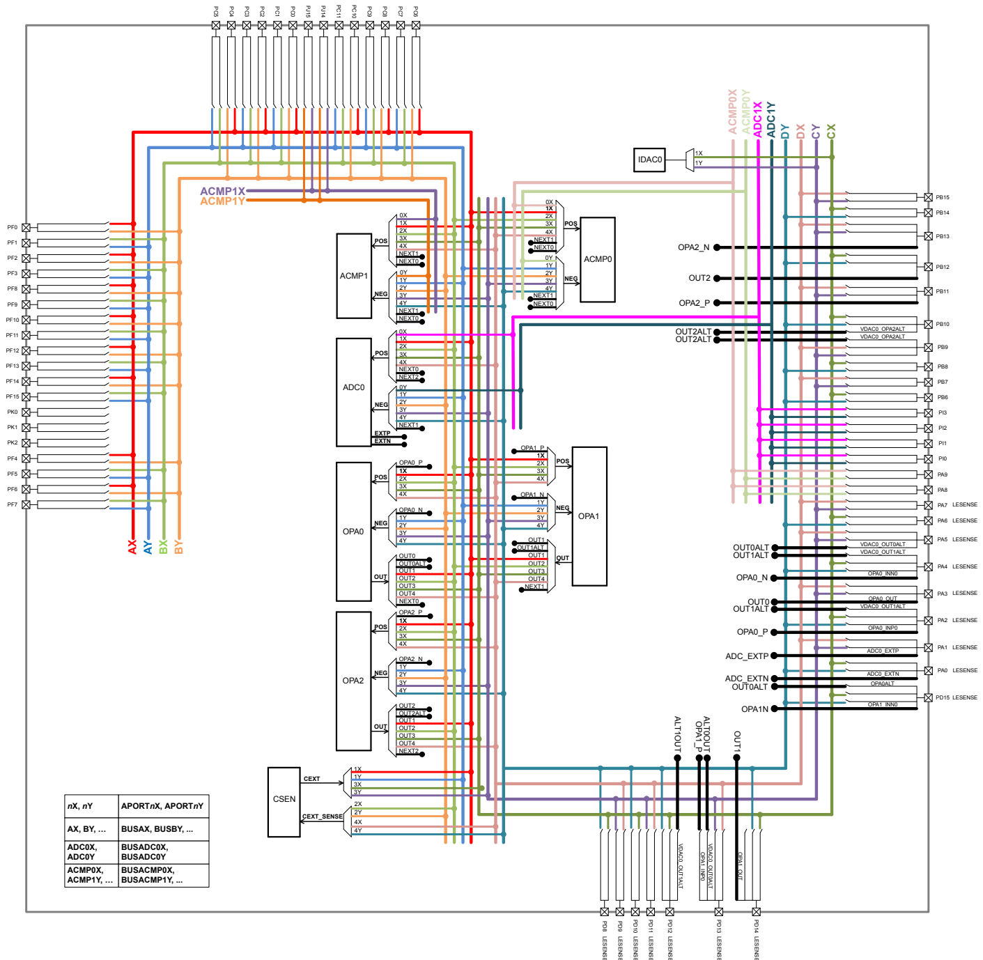
Figure 8.2. APORT Connection Diagram
