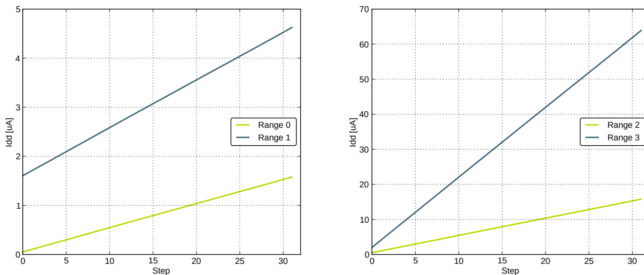
Figure 4.36. IDAC Linearity
