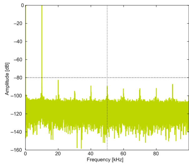
5VDIFF Reference
