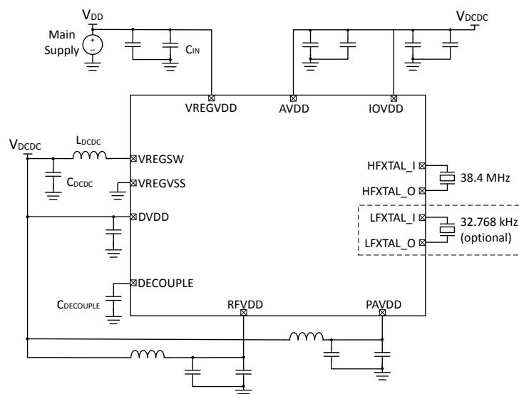
Figure 5.3. EFR32FG22 Typical Application Circuit: DCDC Configuration with PAVDD, RFVDD, AVDD, and IOVDD from DCDC output
