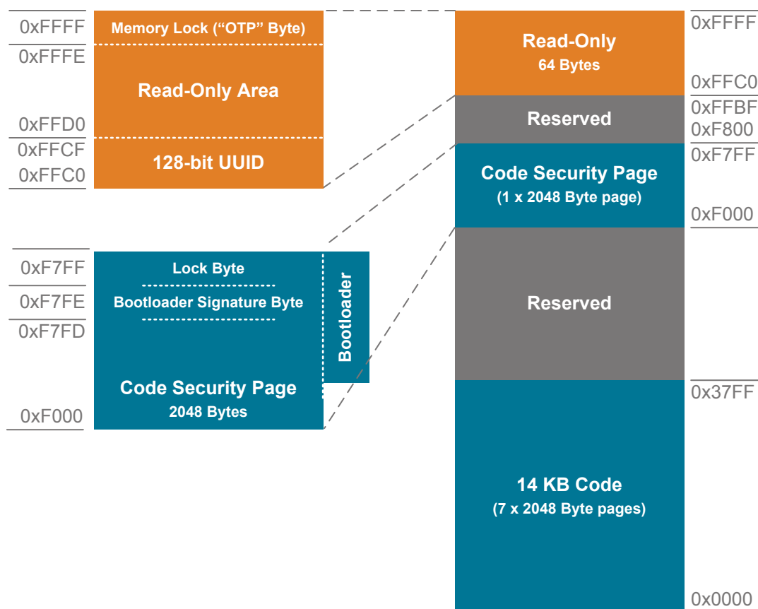
Figure 3.3. Flash Memory Map — 16 KB Devices
