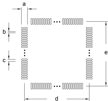
Figure 8.3. TQFP48 PCB Solder Mask
