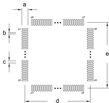
Figure 8.2. TQFP48 PCB Land Pattern
