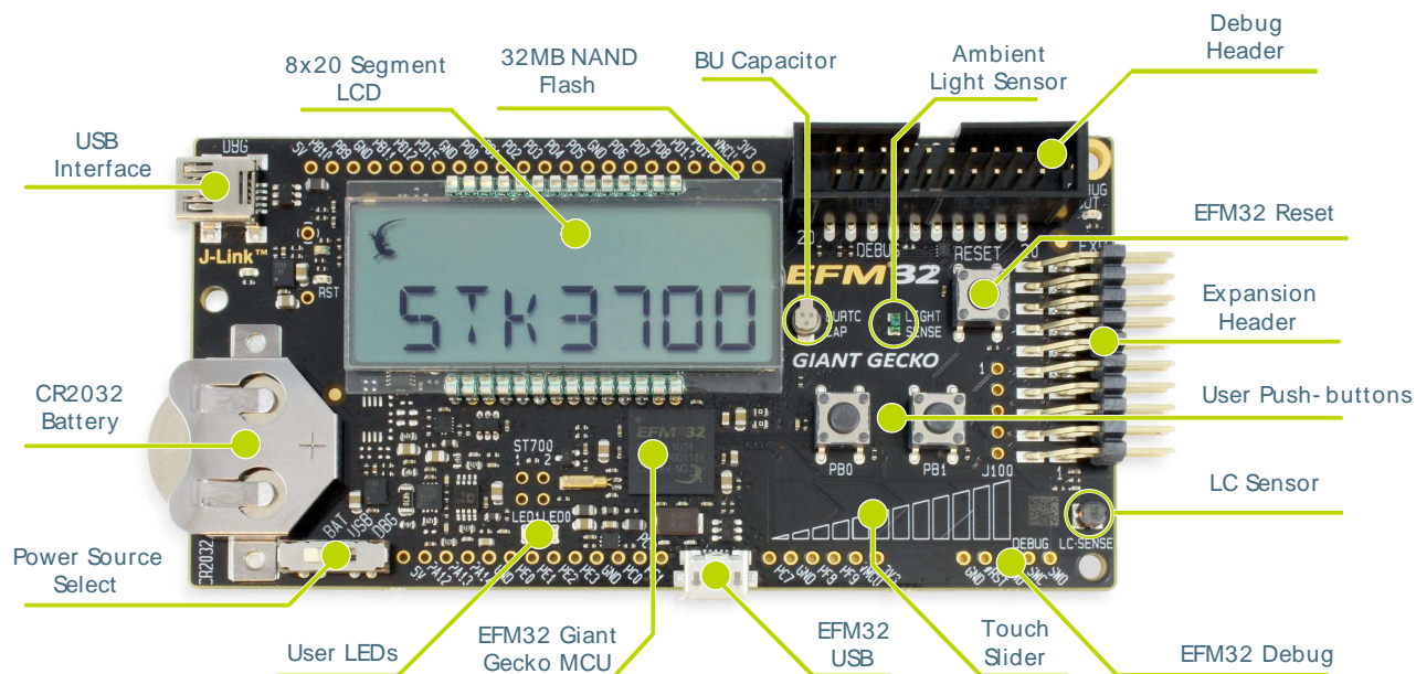
Figure 3.1. EFM32GG-STK3700 hardware layout
