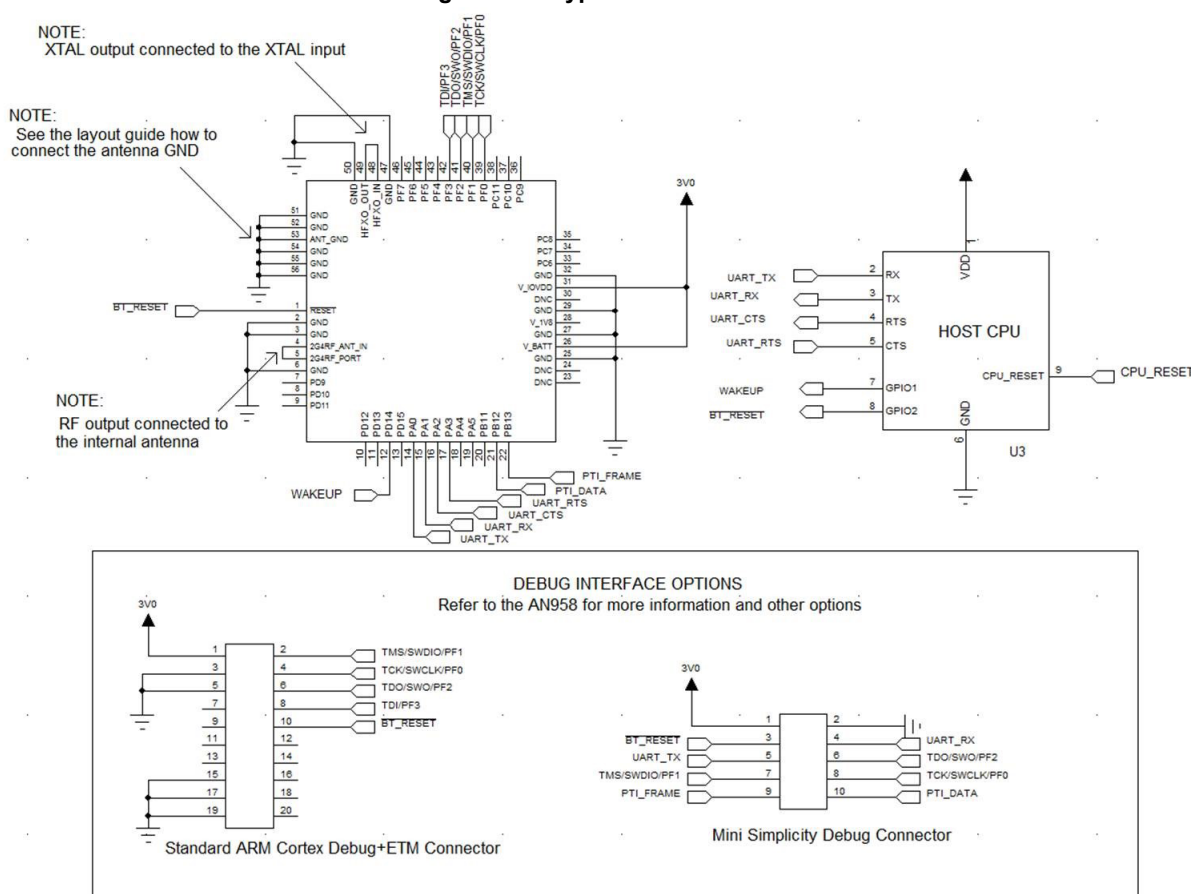
Figure 5.1. Typical Connections
