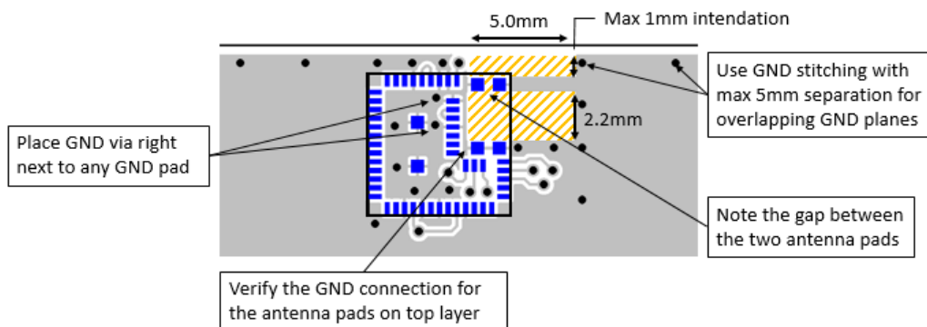
Figure 6.1. BGM111S PCB Top Layer Design
