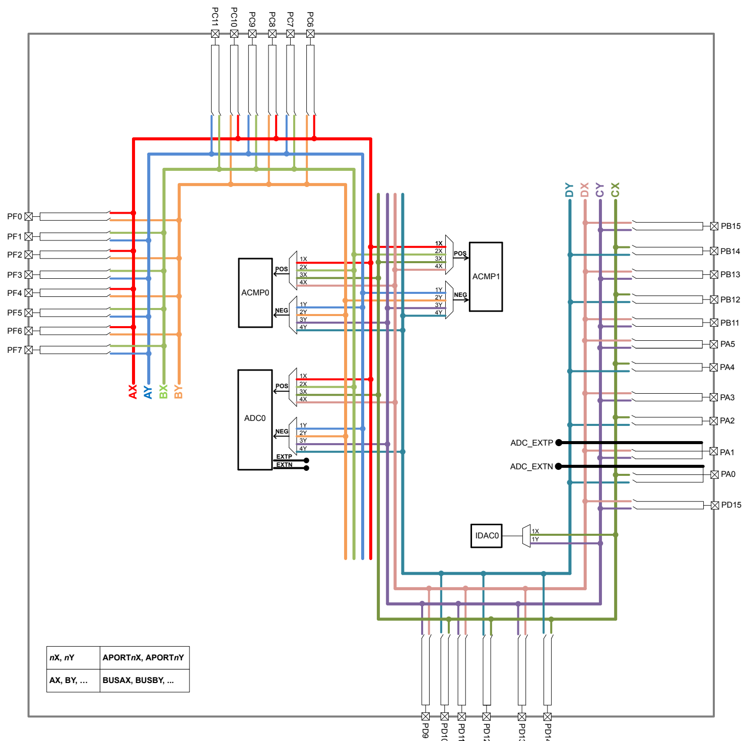
Figure 7.2. BGM11S APORT
