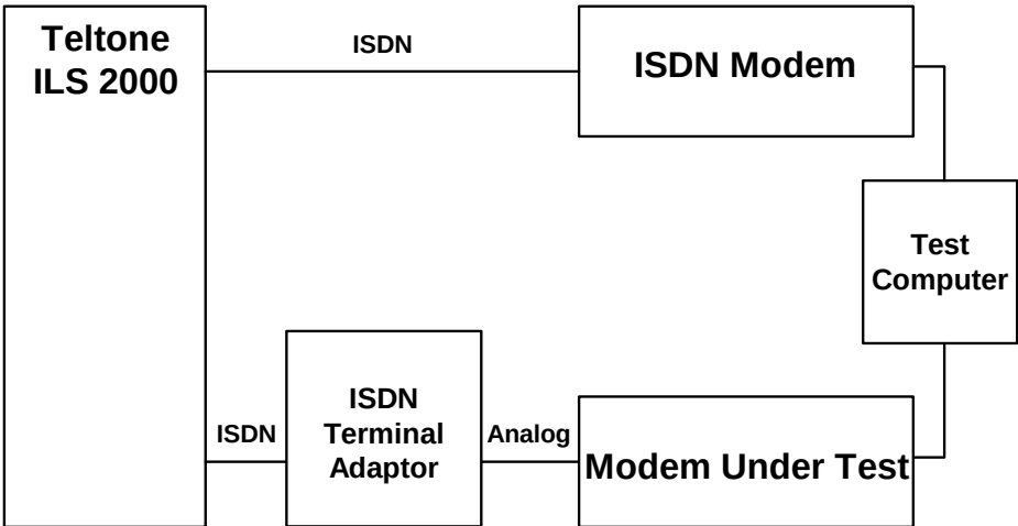
Figure 49. V.90 Modem Functional Test Connection
