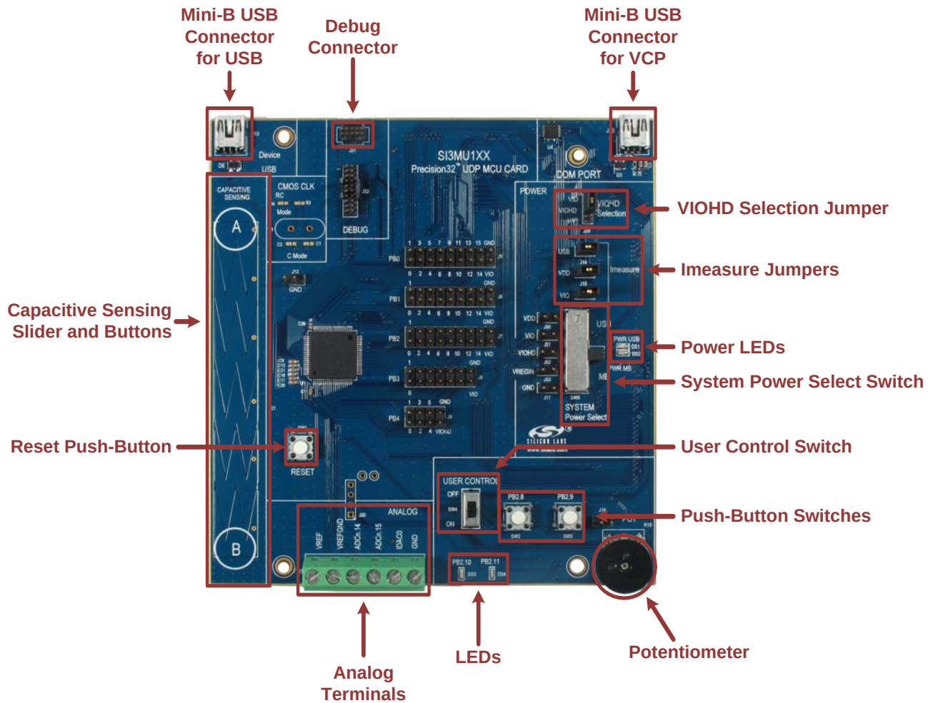
Figure 6. UDP SiM3U1xx MCU Card Features
