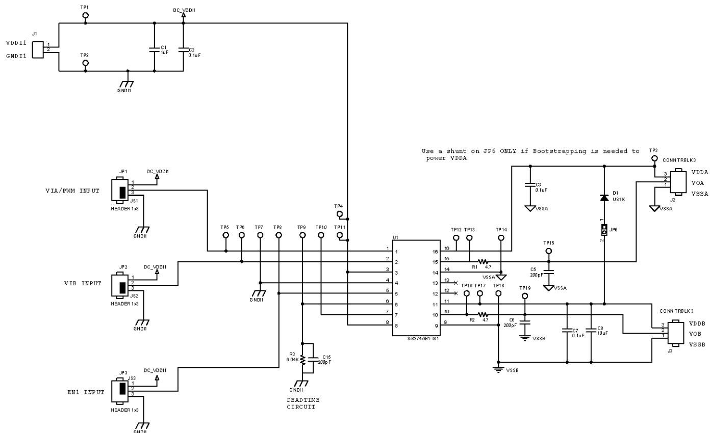
Figure 4.1. Si827x Evaluation Board Schematic (1 of 2)
