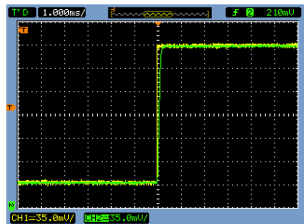
Figure 6: TS1005 Transient Response for R_{ISO} = 50 k \Omega and C_{LOAD} = 500 pF.
