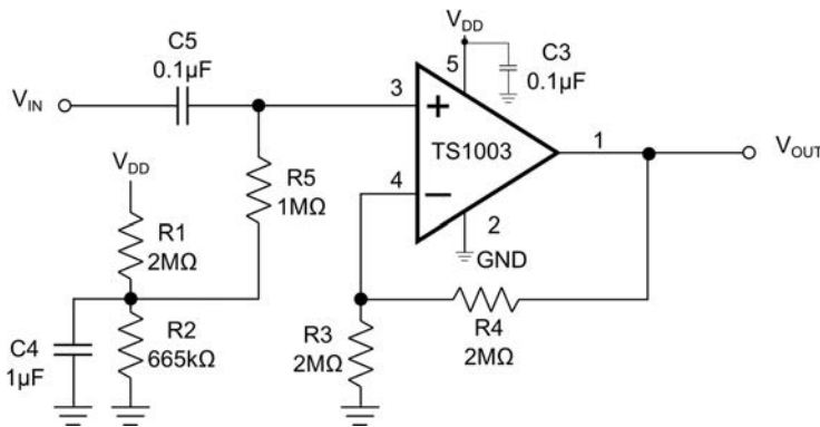
Figure 3. Non-Inverting Configuration
