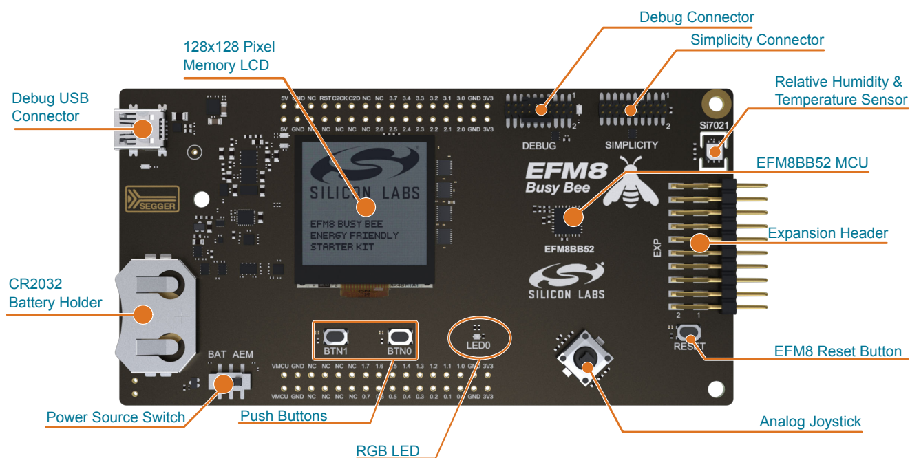
Figure 3.1. BB52-PK5206A Hardware Layout
