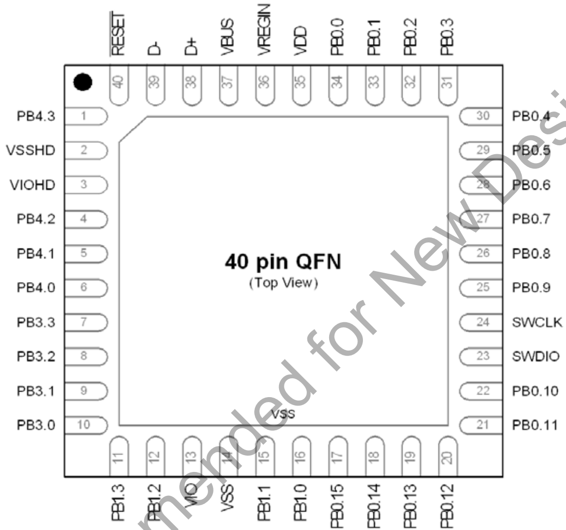
Figure 6.5. SiM3U1x4-GM Pinout
