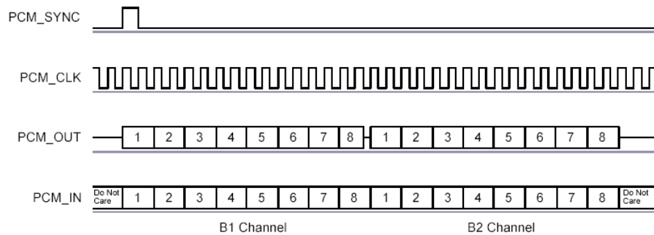
Figure 21: GCI Interface
