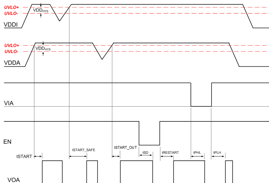
Figure 2.5. Si823H7 (Delayed Startup Time of t_{\text{START\_SAFE}} ) Device Behavior During Normal Operation and Shutdown
