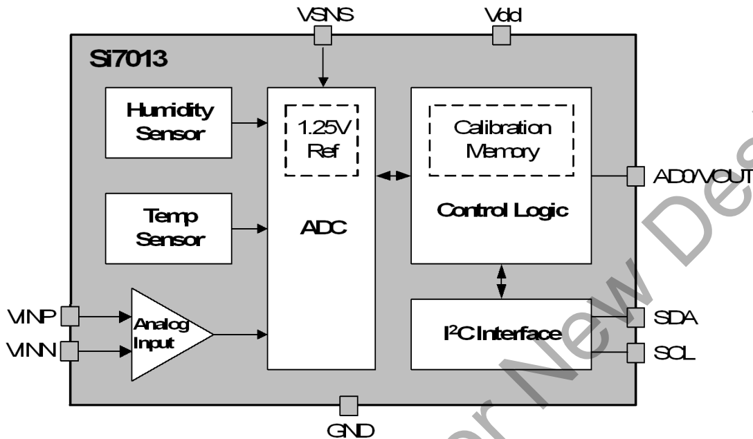
Figure 8. Si7013 Block Diagram
