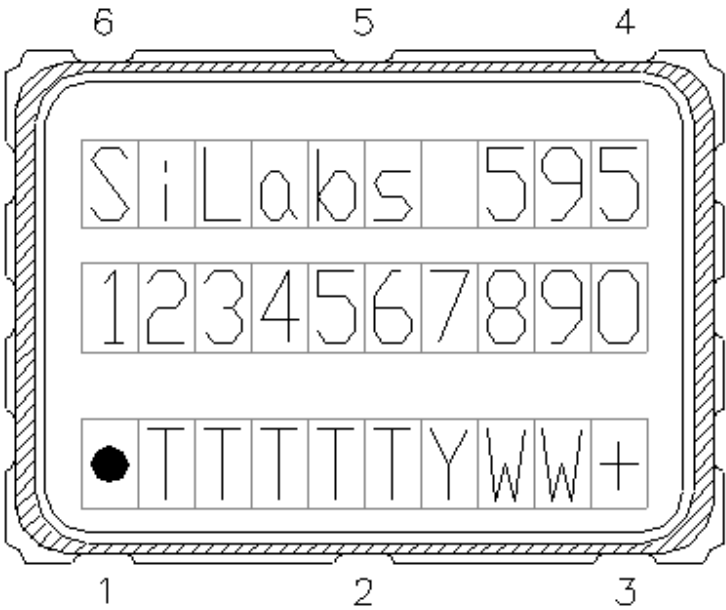
Figure 6. Mark Specification Table 16. Si595 Top Mark Description
