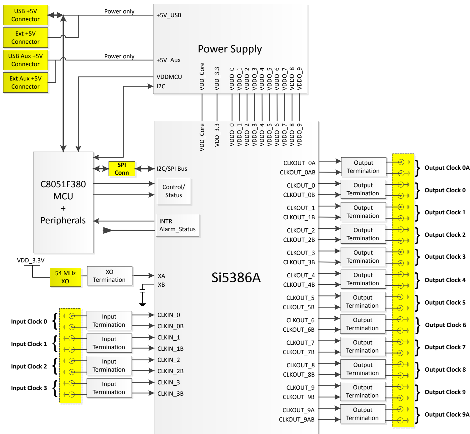
Figure 1.1. Functional Block Diagram of Si5386A-E-EB
