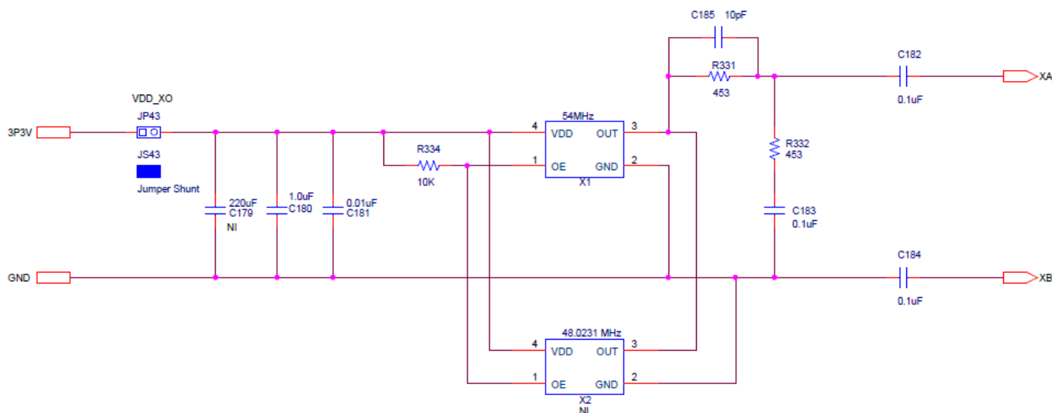
Figure 4.1. External Reference Input Circuit
