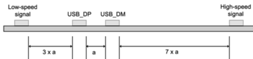
Figure 19 Spacing for Low-speed and High-speed signals around USB_DP/USB_DM
