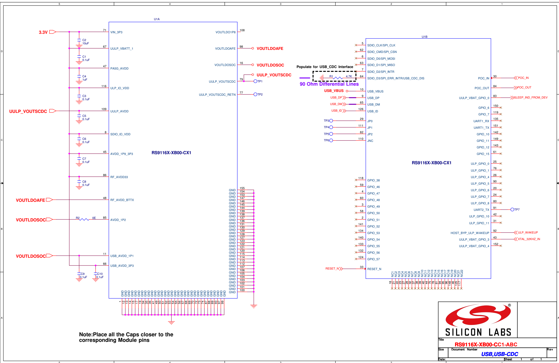
Figure 17. USB Schematics
