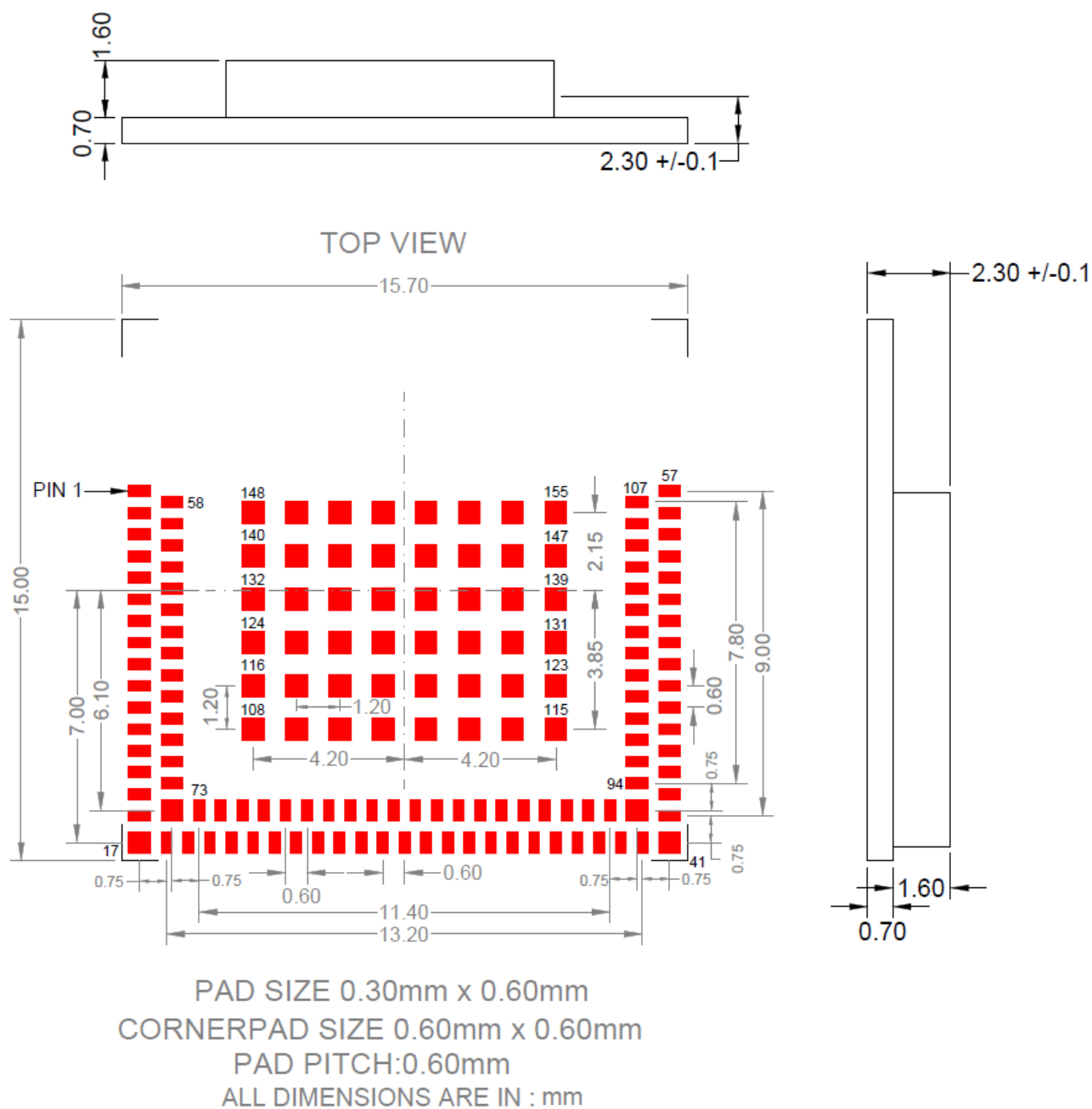
Figure 46. Package Outline
