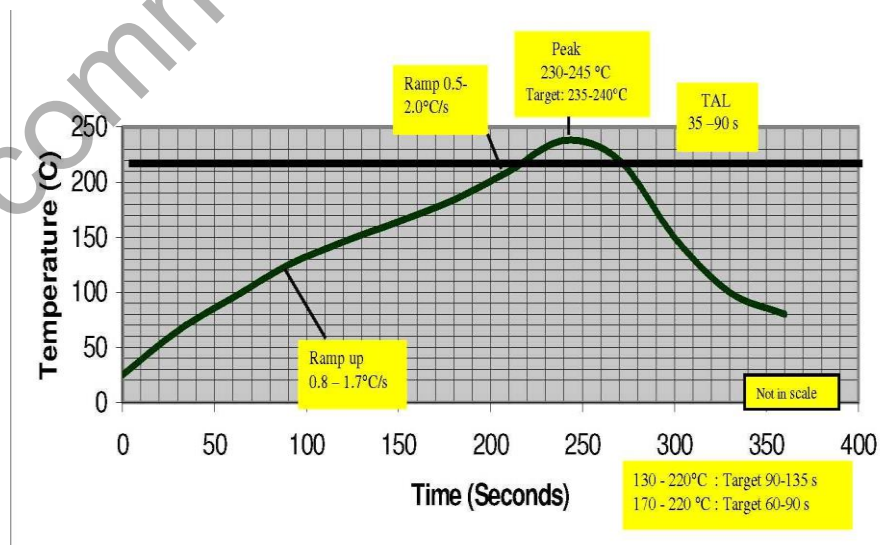
Figure 7: Reflow Diagram
