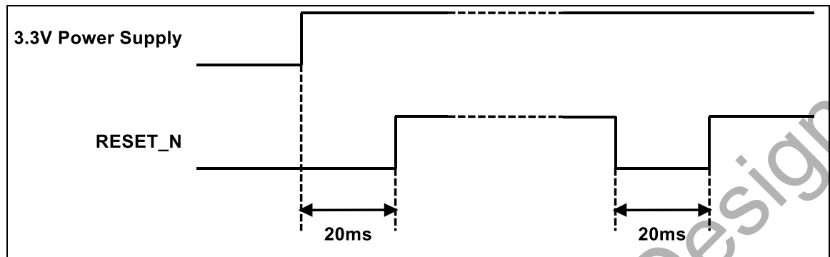
Figure 12: Reset Timing
