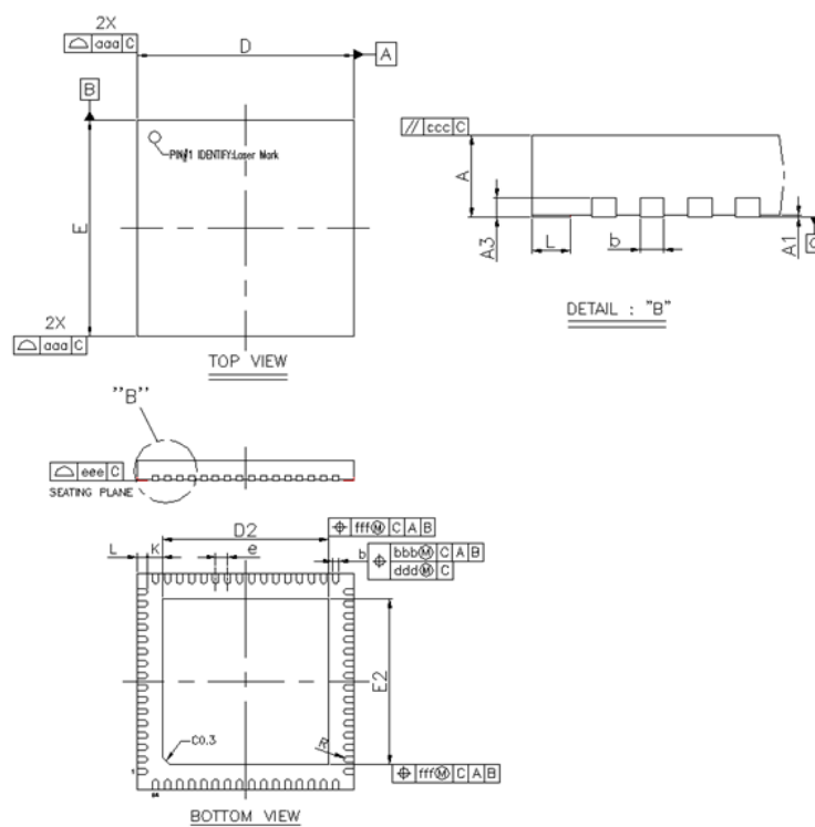
Figure 5.3. QFN64
