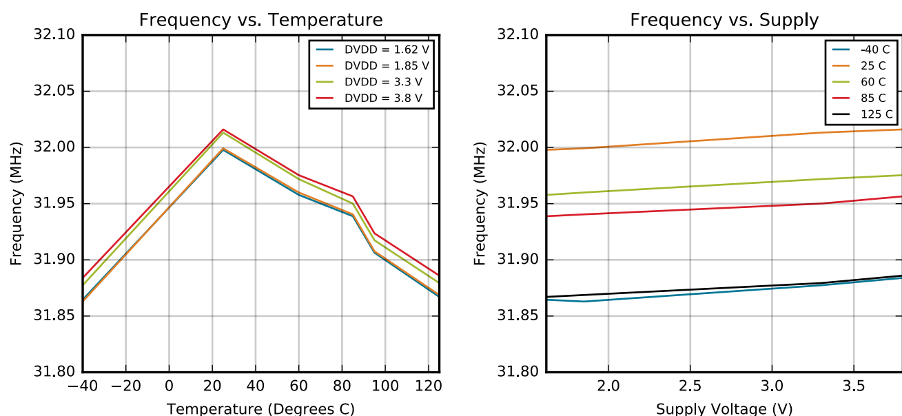
Figure 4.10. HFRCO and AUXHFRCO Typical Performance at 32 MHz
