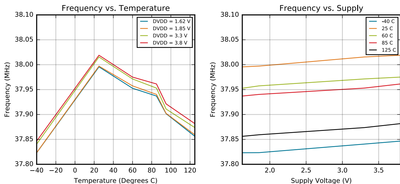
Figure 4.9. HFRCO and AUXHFRCO Typical Performance at 38 MHz
