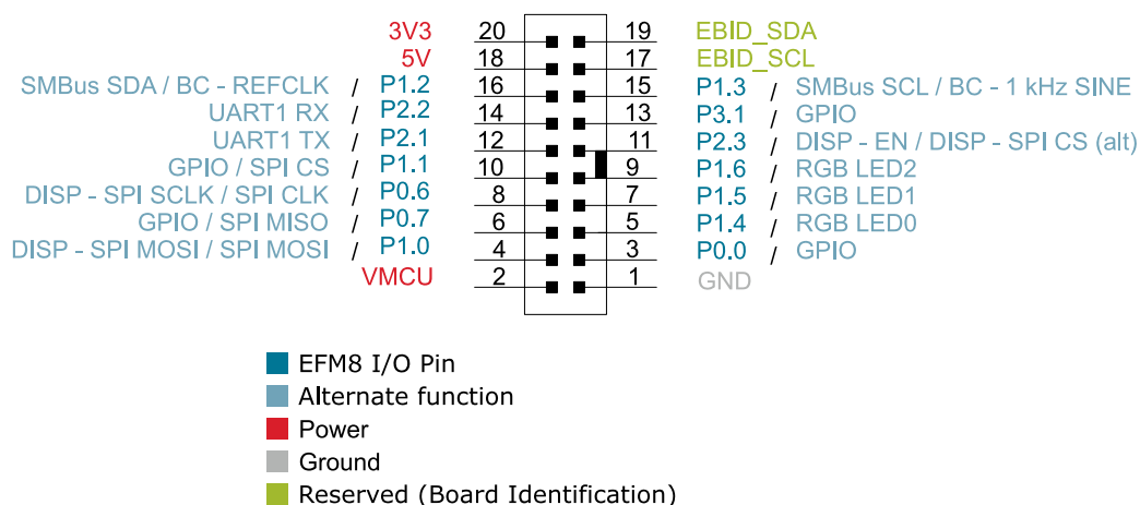
Figure 6.2. Expansion Header
