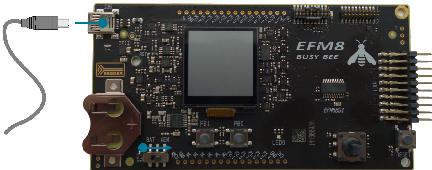
Figure 1.1. Hardware Setup
