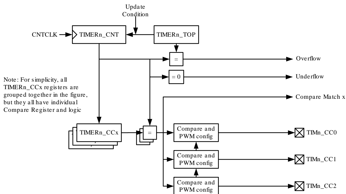
Figure 19.15. TIMER Block Diagram Showing Comparison Functionality
