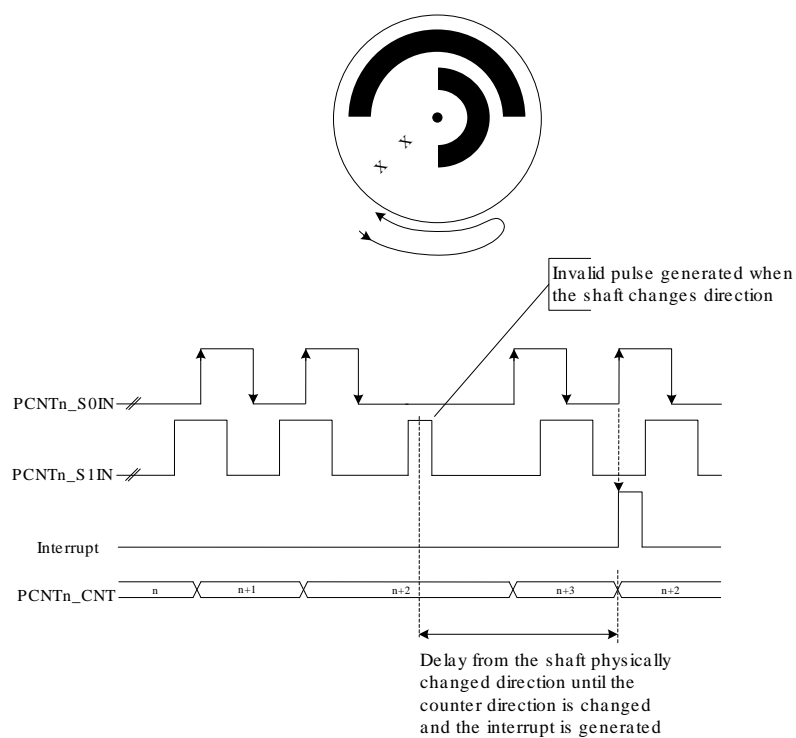
Figure 22.3. PCNT Direction Change Interrupt (DIRCNG) Generation
