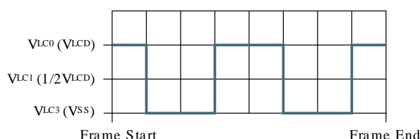
Figure 29.7. LCD 1/2 Bias and Duplex Multiplexing - LCD_SEG0
