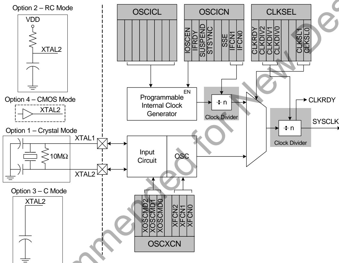
Figure 27.1. Oscillator Options
