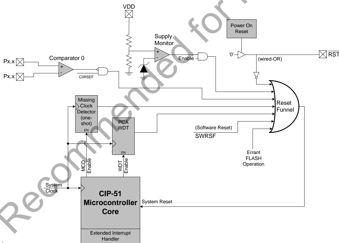
Figure 25.1. Reset Sources
