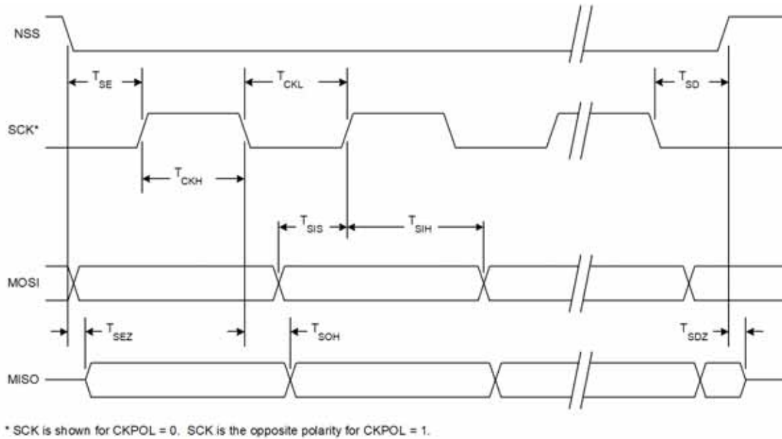
Figure 16.8. SPI Slave Timing (CKPHA = 0)
