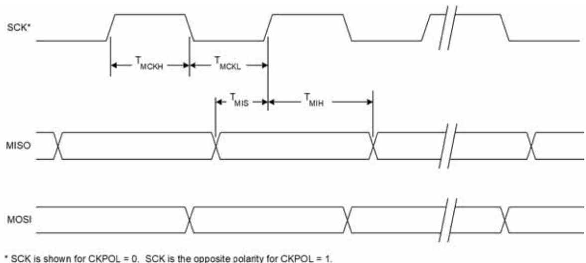
Figure 16.6. SPI Master Timing (CKPHA = 0)
