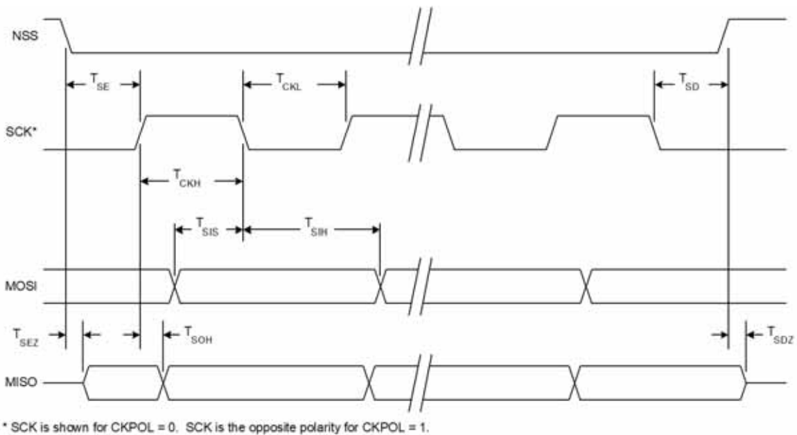
Figure 16.9. SPI Slave Timing (CKPHA = 1)
