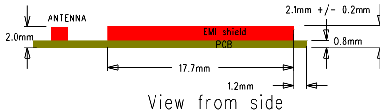
Figure 4: Physical dimensions
