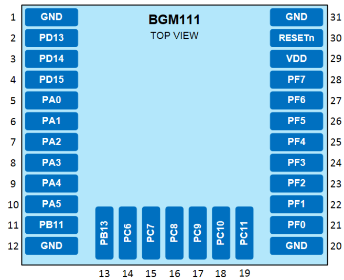
Figure 7.1. BGM111 Pinout
