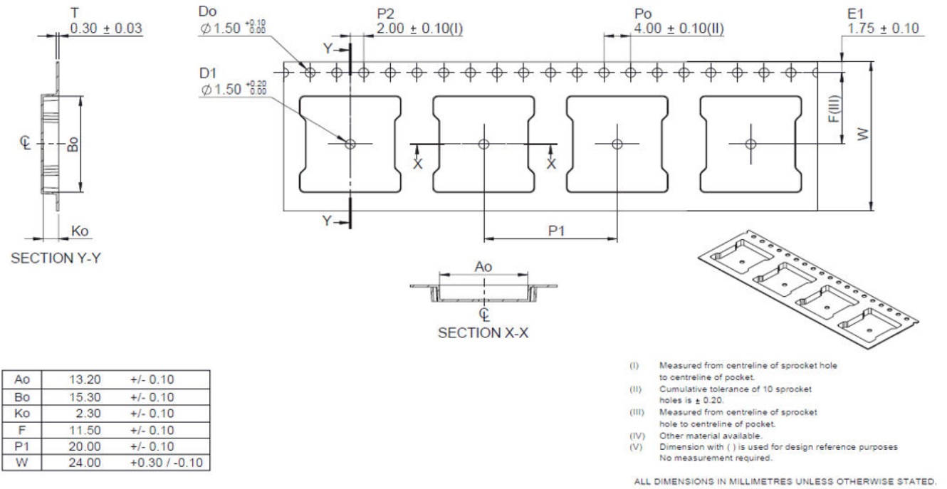
Figure 9.2. Tape Information
