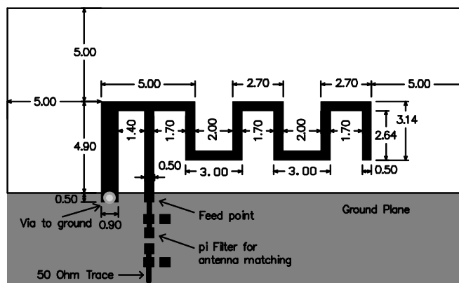
Figure 8 - Trace Antenna (dimensions in mm)
