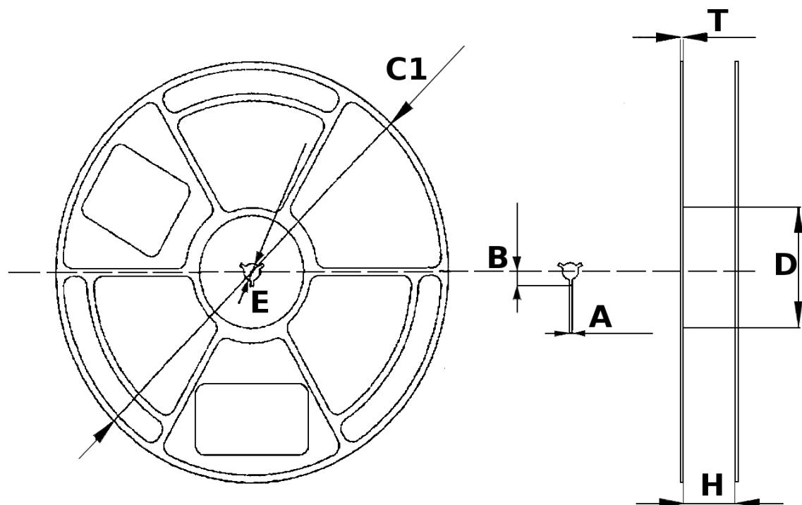
Figure 8 - Reel Specifications
