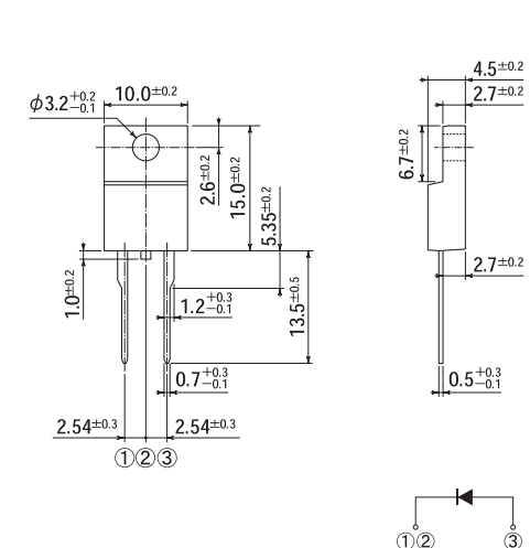
J1 Package: SC-91A
