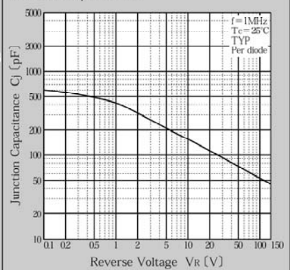
Junction Capacitance
