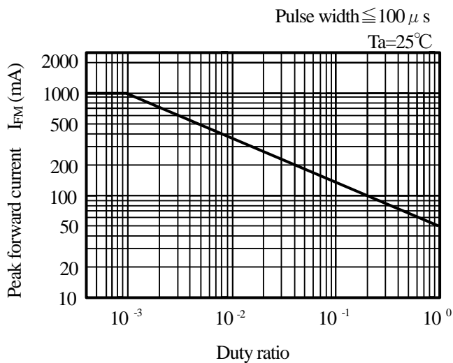
(Fig. 5) Peak forward current vs. Duty ratio
