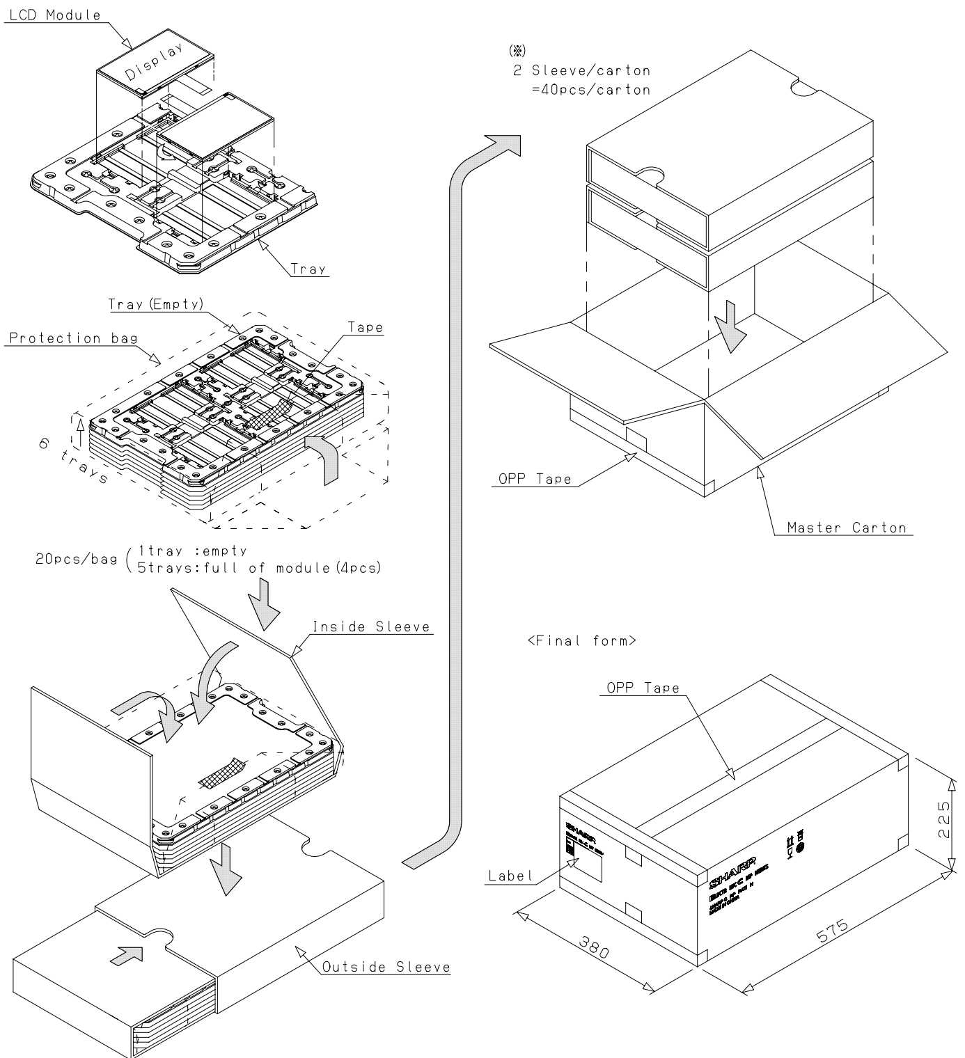
Fig 2. Packing form
