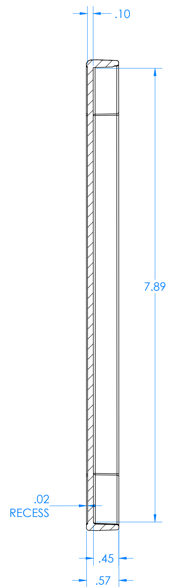
SECTION E-E
