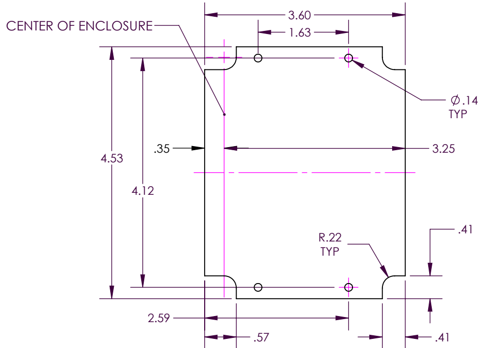
SMALL CIRCUIT BOARD FOR BOTTOM
