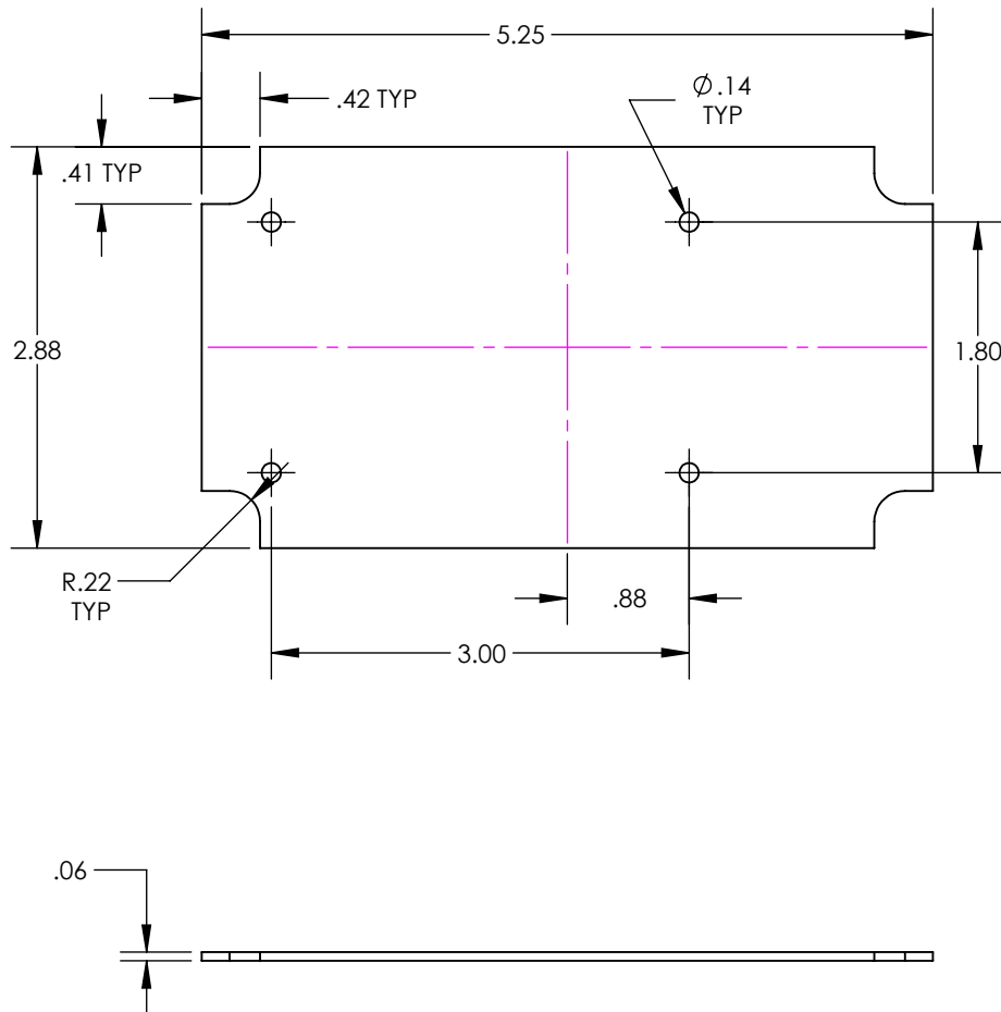
CIRCUIT BOARD FOR BOTTOM
