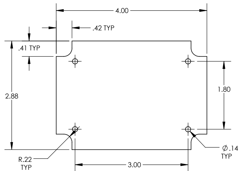
CIRCUIT BOARD FOR BOTTOM
