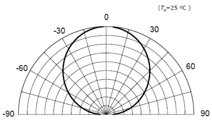
Radiation Diagram
