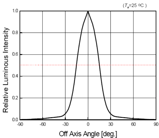
Radiation Diagram
