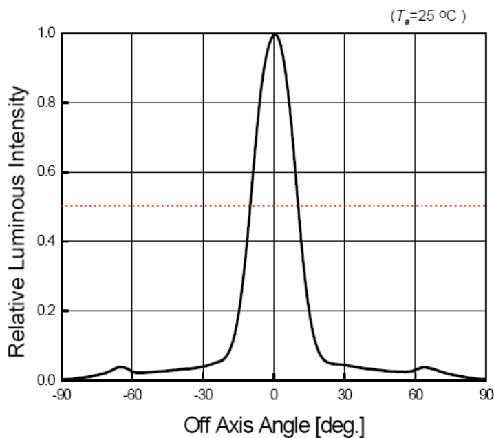
Radiation Diagram
