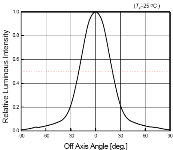
Radiation Diagram
