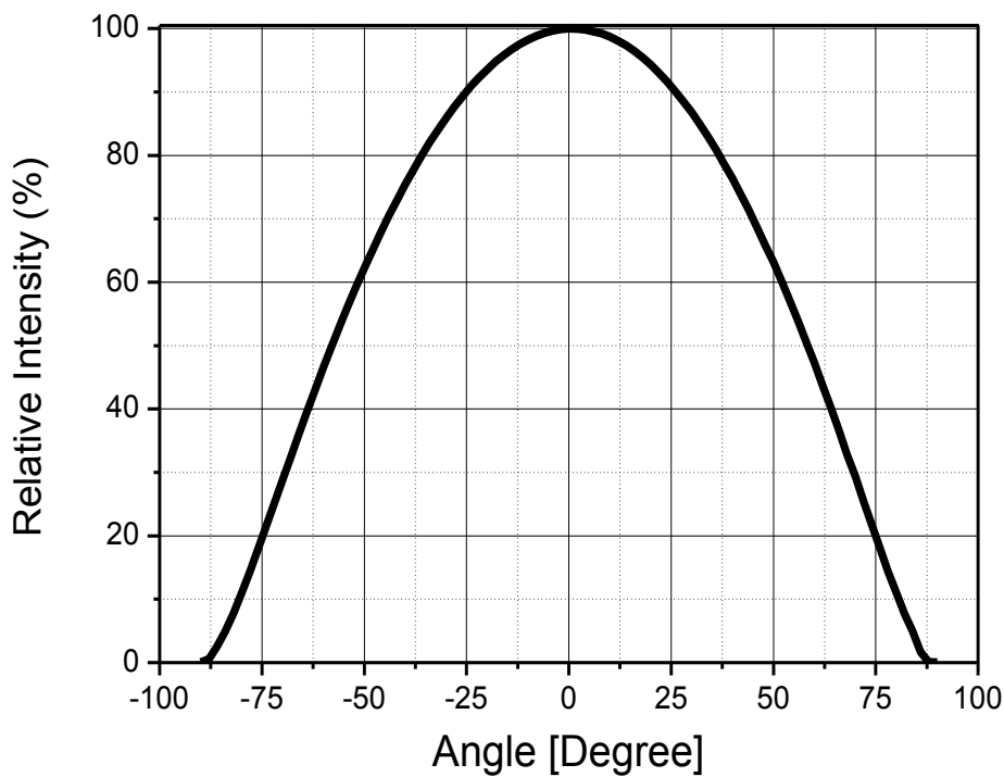
Fig 2. Radiant Pattern, T_j = 25^{\circ}\text{C} , I_F = 32\text{mA}
