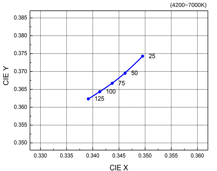
Fig 8. Chromaticity Coordinate vs. Junction Temperature, I_F=32\text{mA}
