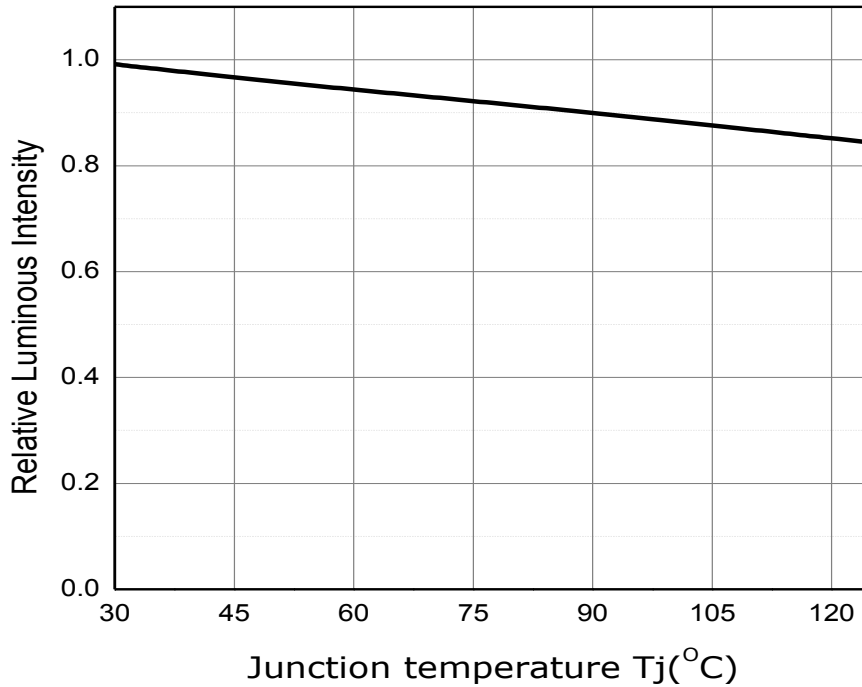
Fig 6. Junction Temperature vs. Relative Luminous Intensity, I_F=32\text{mA}
