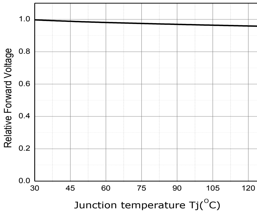
Fig 7. Junction Temperature vs. Relative Forward Voltage, I_F=32\text{mA}
